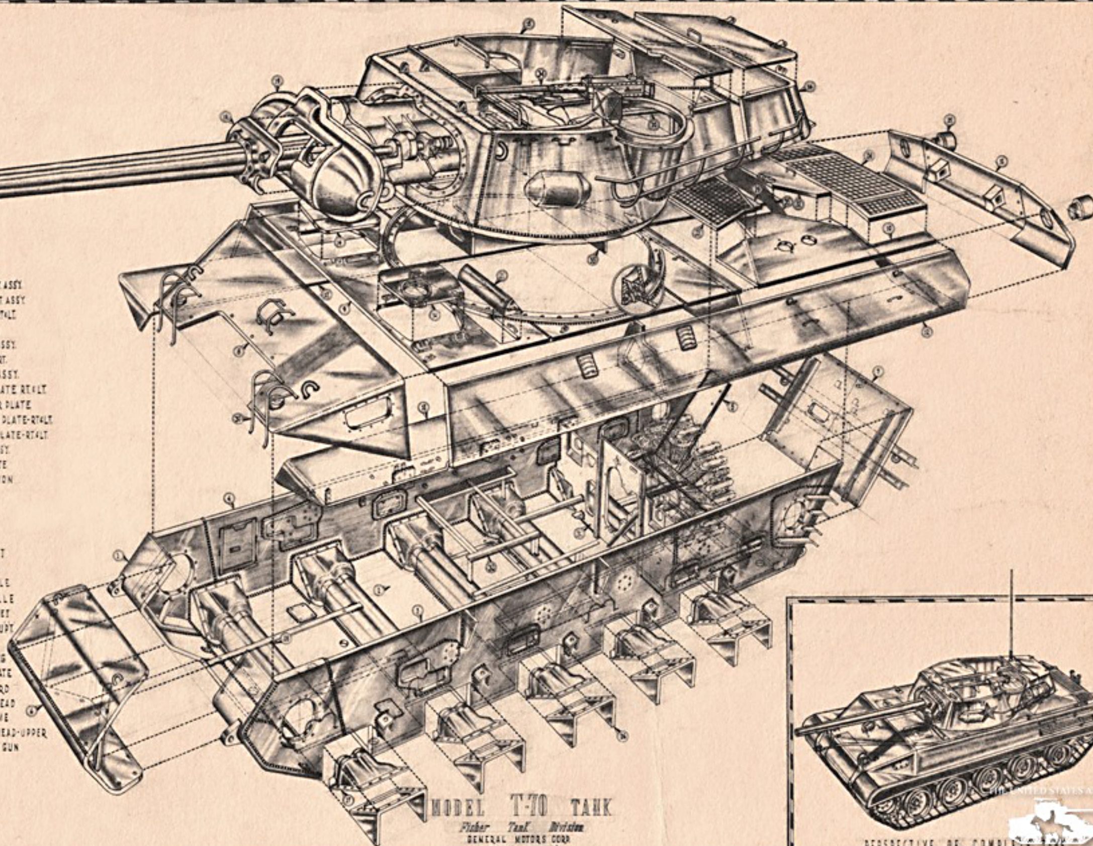
PERSPECTIVE OF COMPLETE TANK
