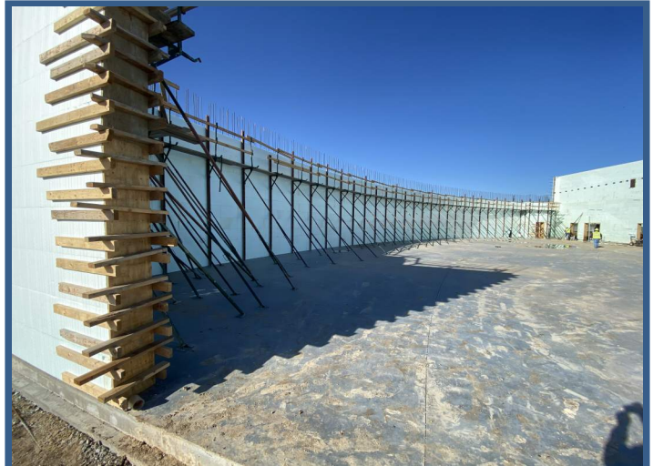
ICF at Main Exhibit Hall Ready for Concrete
